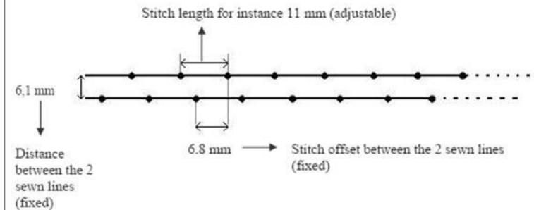
Stich and sewn line dimensions:
